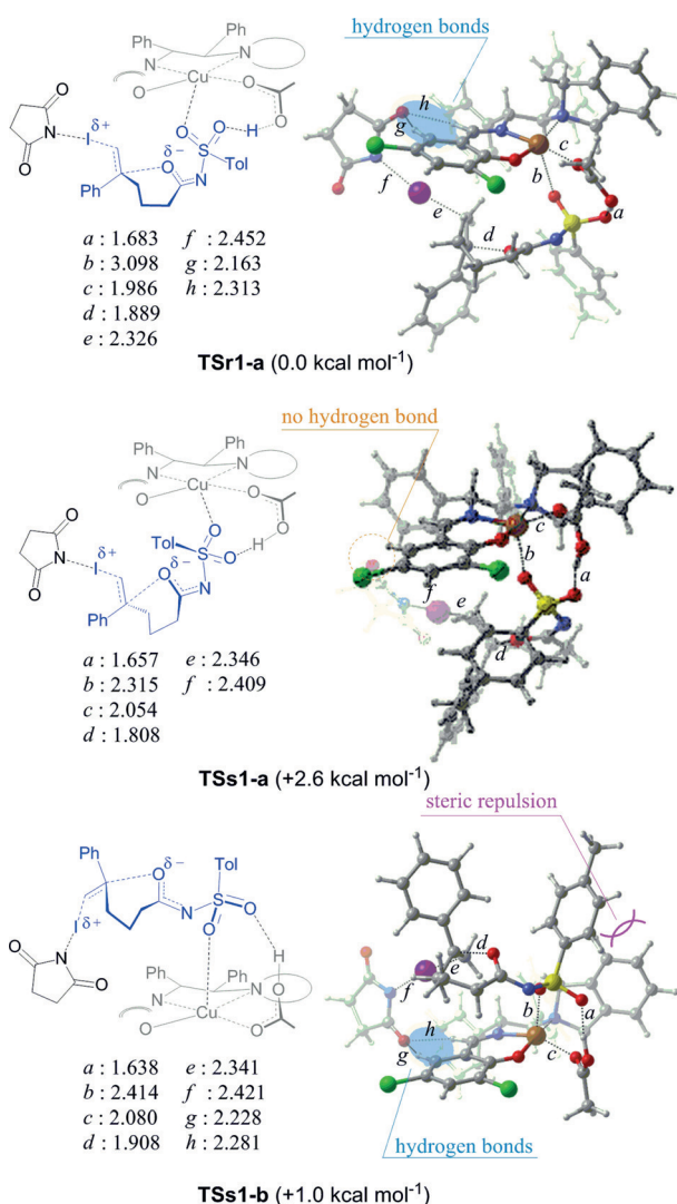
Figure 5. 3D structures, representations, and relative energies of diastereomeric TSs ( TSr1-a , TSs1-a , and TSs1-b ). Bond lengths are shown in Å.
